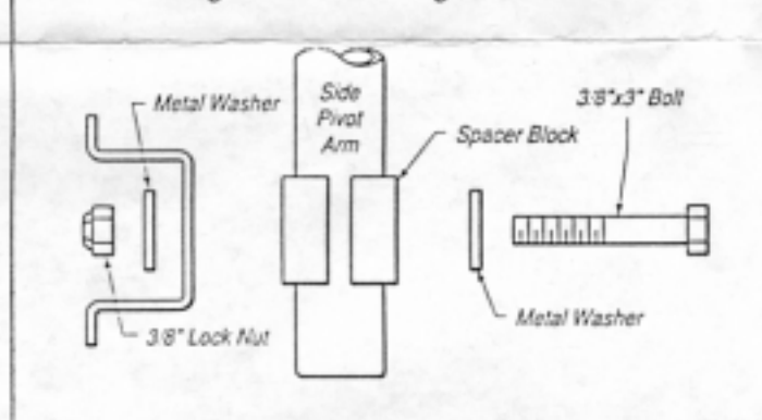
Figure 3 - Assembly of Support Arms to Pivot Arms
