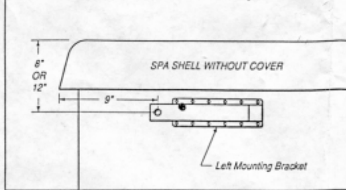
Figure 2 - Attaching Pivot Arms
